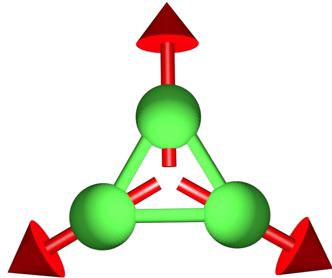
Frustrated magnetism
