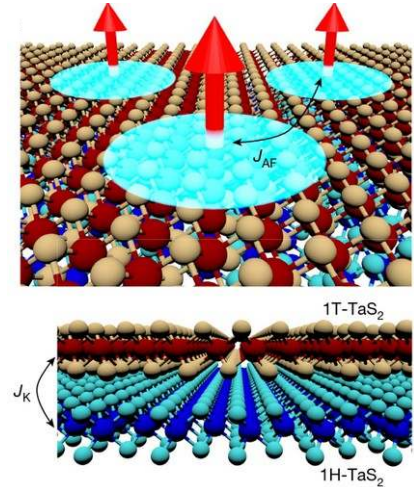
1H-1T \text{TaS}_2
